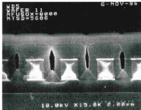
Figure 3.28: Microchip fabrication. Plasma-enhanced chemical vapor deposition.
