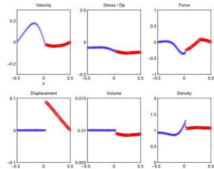
Figure 8.10: Fluid-solid interactions in 1D. Profile of velocity, stress, body force, displacement, volume and density at t = 2 . Fluid on the left, solid on the right.
