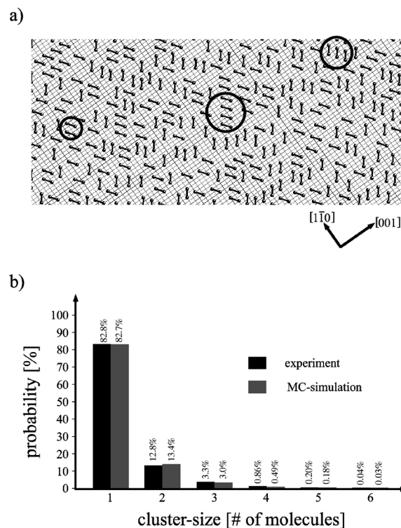
Fig. 3. (a) Monte Carlo simulation for PVBA on Pd(110) film growth with site-blocking and immobile adsorption. Circles mark molecular clusters which are similarly found in the STM images in Fig. 2, where an extrinsic precursor mechanism is operative. (b) Comparison of cluster size distribution obtained from STM images and Monte Carlo simulations. There is no significant difference in the ordering, indicating that the extrinsic precursor mechanism with the molecules' adsorption does not improve the film ordering for the present system.
