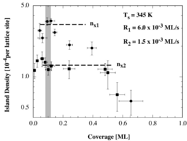
Figure 1. Island densities versus coverage for two different fluxes ( 1.5 \times 10^{-3} ML/s and 6.0 \times 10^{-3} ML/s) at a substrate temperature of 345 K.
