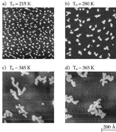
Figure 2. STM images characterizing the saturation island densities for the submonolayer growth of Cu on Ni(100) at different growth temperatures and fixed deposition rate ( 1.5 \times 10^{-3} ML/s) and coverage (0.1 ML).
