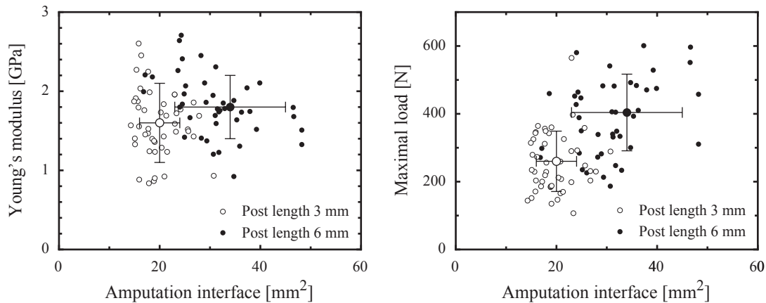
Figure 9. Larger teeth are selected to place the longer posts. Therefore, especially the maximal load seems to depend on the post length.
